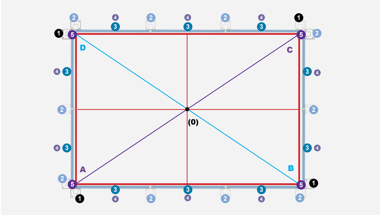
1 Angle pillars
