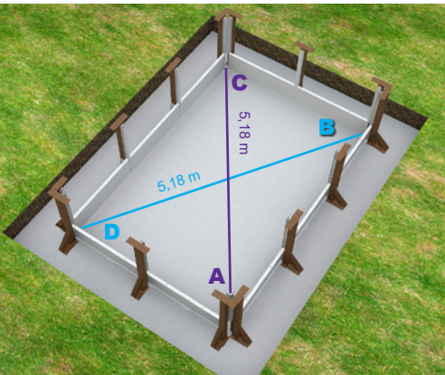
4 Triangular reinforcement
