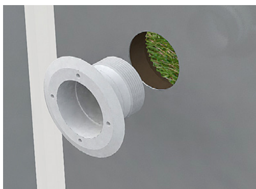
The outlet nozzle is placed in the hole conceived for this purpose.
